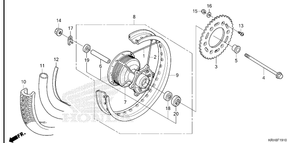
REAR WHEEL
