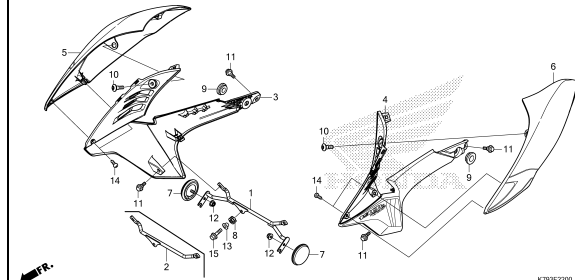
SHROUD
