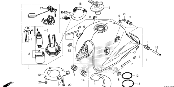
FUEL TANK
