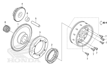
STARTING CLUTCH
